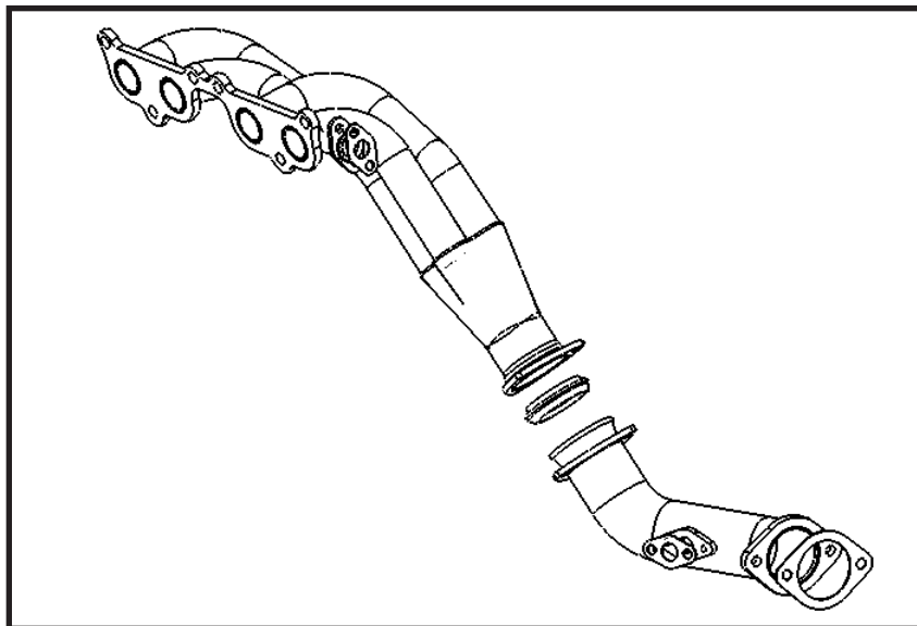
Figure 1 ( Assembled view )
